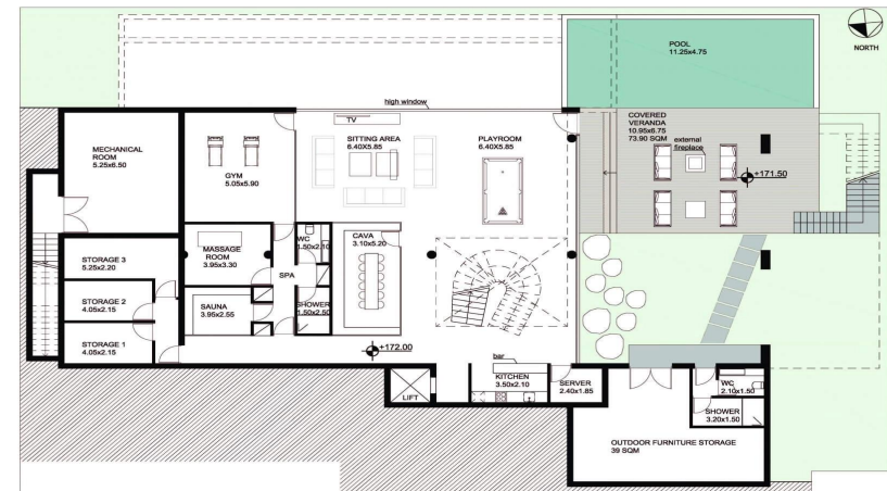
BASEMENT PLAN
