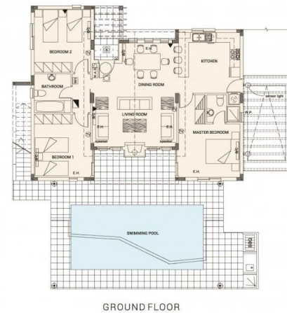
3 BEDROOM VILLA
