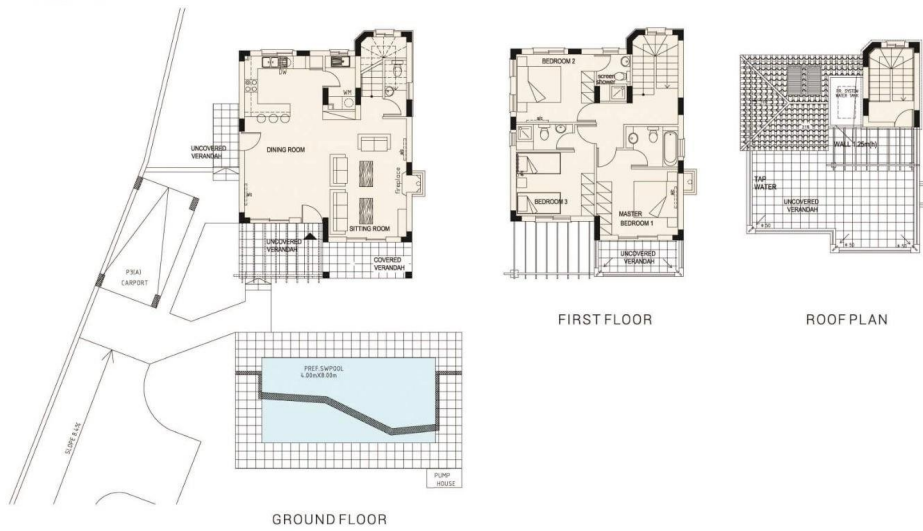
3 BEDROOM VILLA
