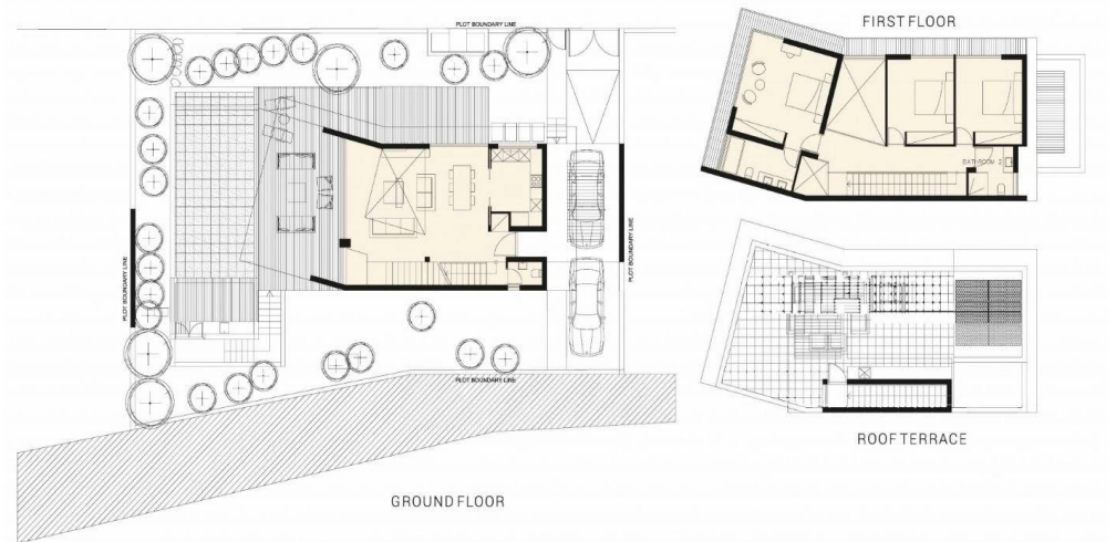
3 BEDROOM VILLA
