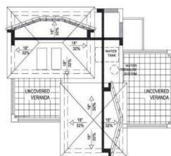
ROOF PLAN
