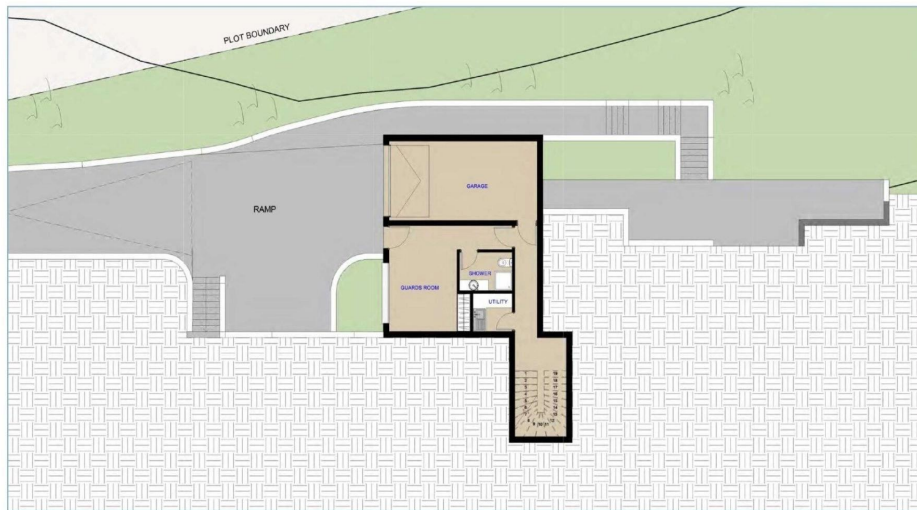
PRELIMINARY LOWER GROUND FLOOR PLAN
