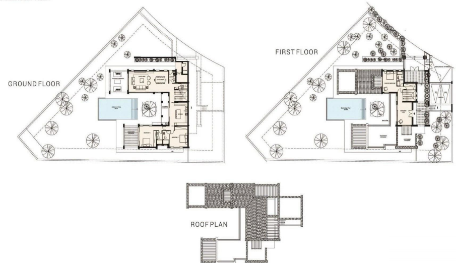
3 BEDROOM VILLA
