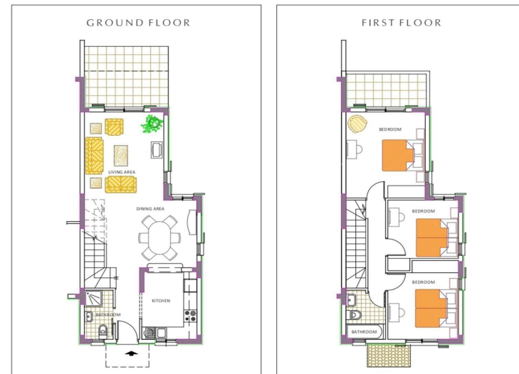
TOWNHOUSE M01
