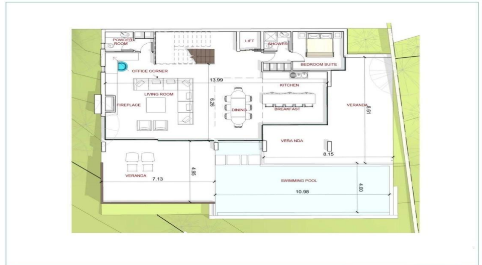
PRELIMINARY GROUND FLOOR PLAN
