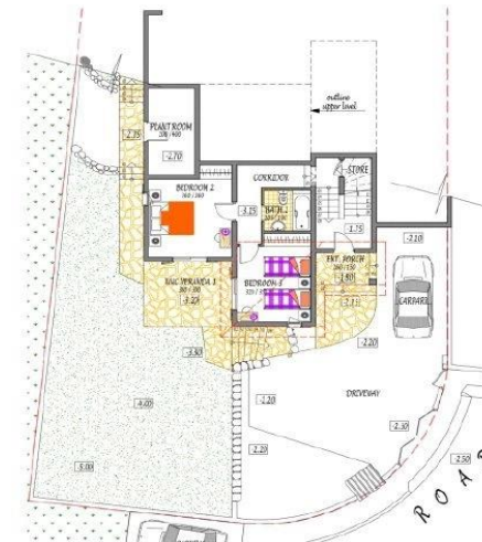
PRELIMINARY GROUND FLOOR
