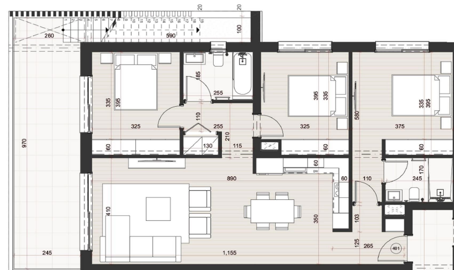
Ground Floor
