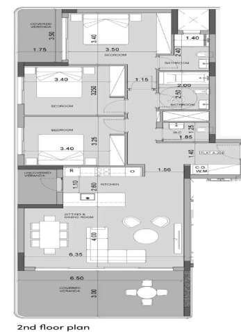
2nd floor plan
