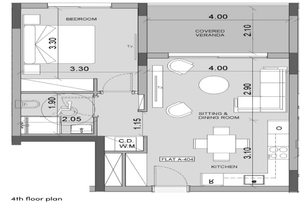
4th floor plan
