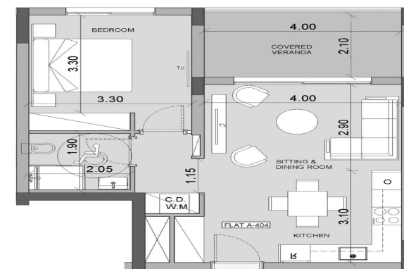
4th floor plan
