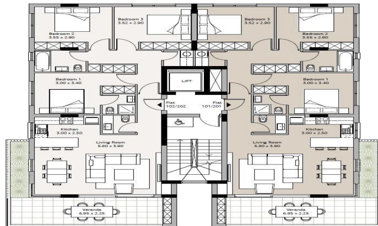
Flat 101, 102, 201, 202
