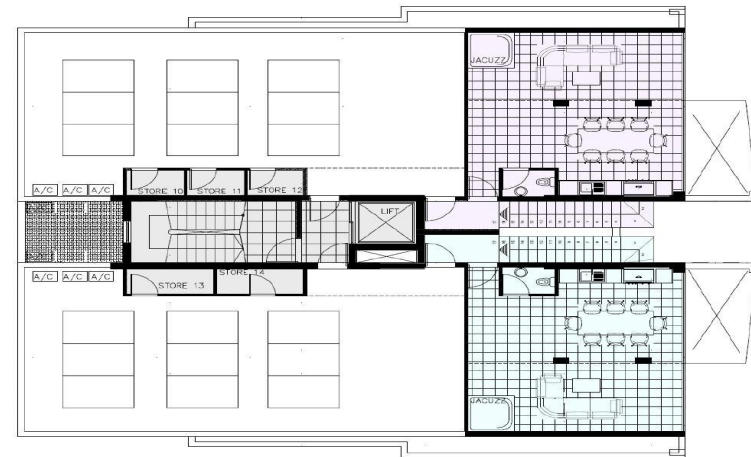
5 floor
