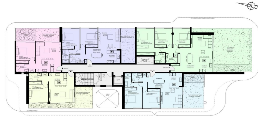
2nd floor
