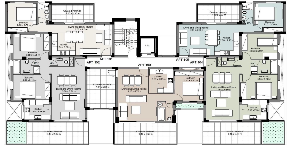
First Floor
