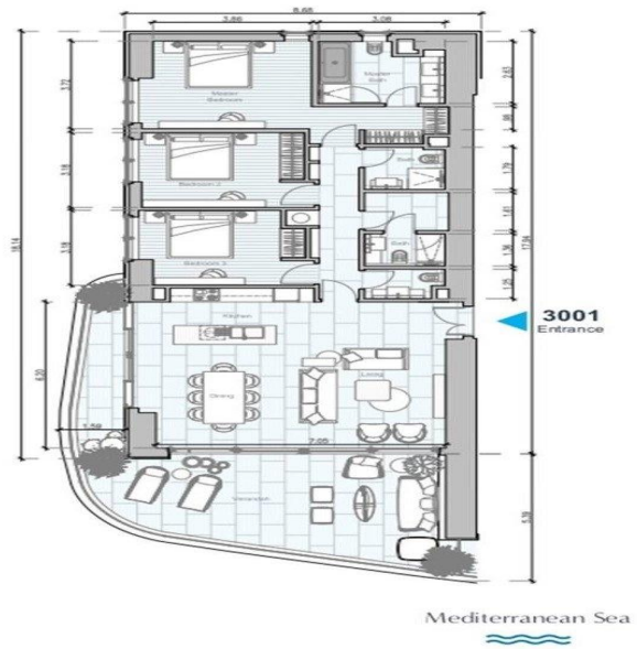
Preliminary Apartment Plan
