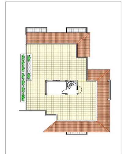
ROOF PLAN
