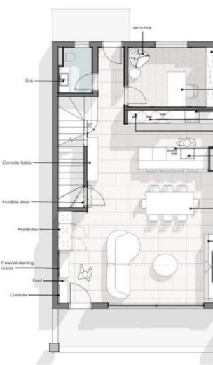
1 Furniture layout Ground floor 1:65
