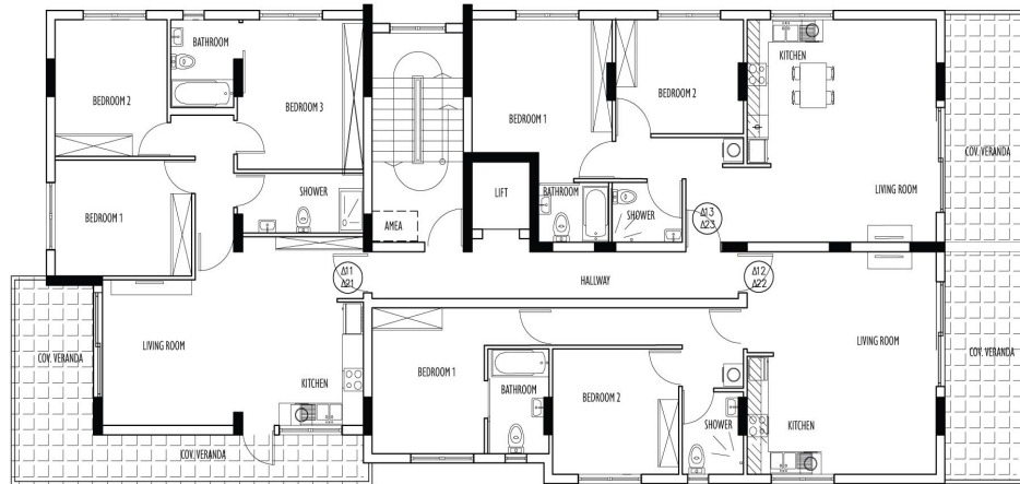
First & Second Floor Plan
