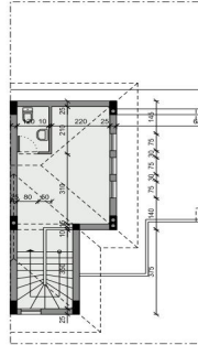
ATTIC FLOOR PLAN
