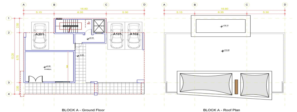
BLOCK A - Ground Floor
