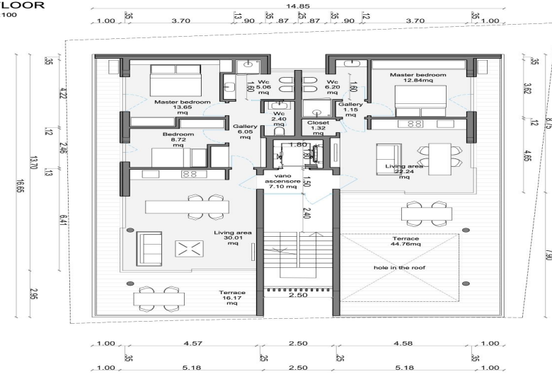
3th FLOOR Scale 1:100
