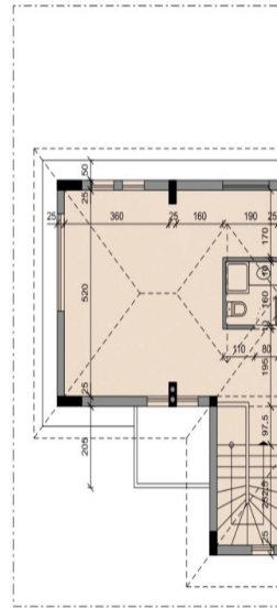
ATTIC FLOOR PLAN
