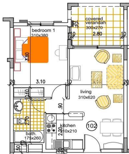
APARTMENT PLAN
