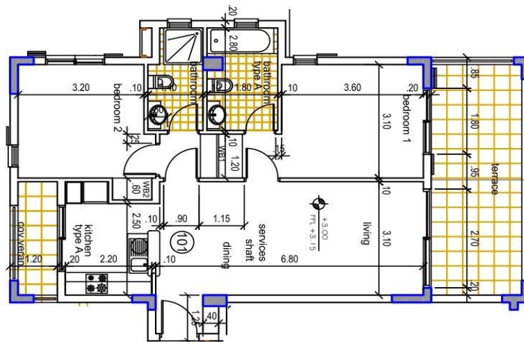
APARTMENT PLAN
