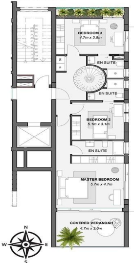
3RD FLOOR
