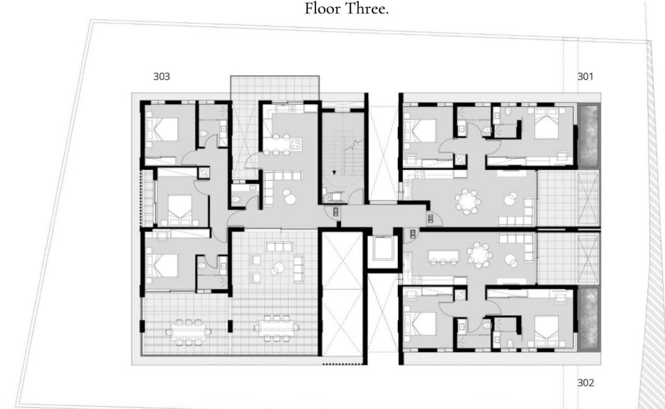
Floor Three.
