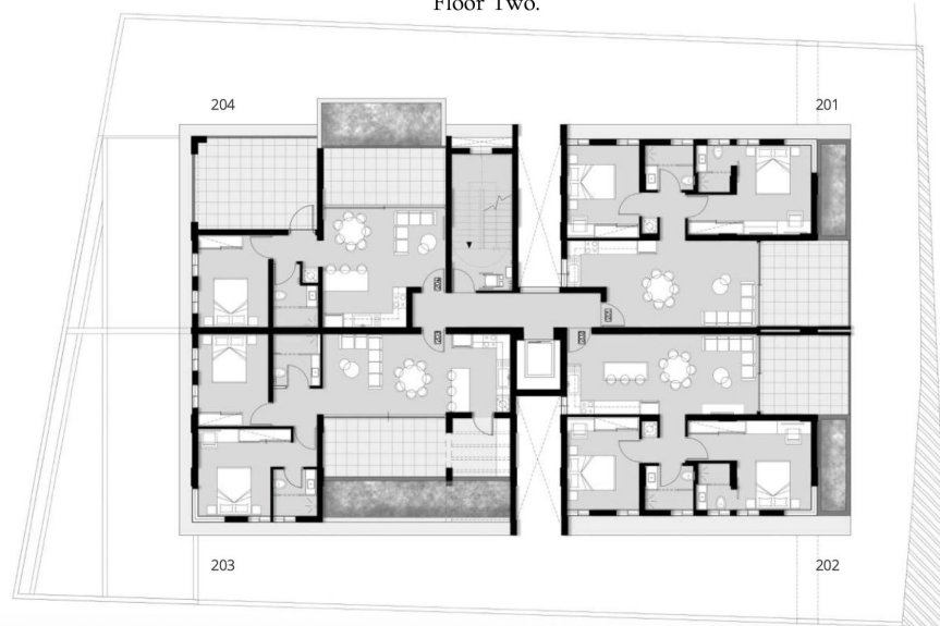
Floor Two.
