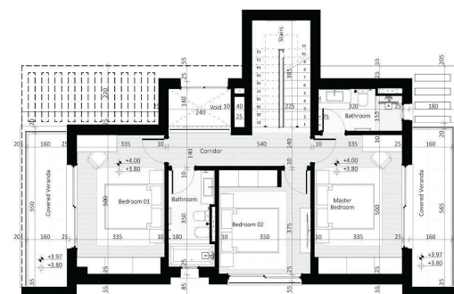
Villa C Total - 349,80 m2 Plot area - 530,00 m2 First floor
