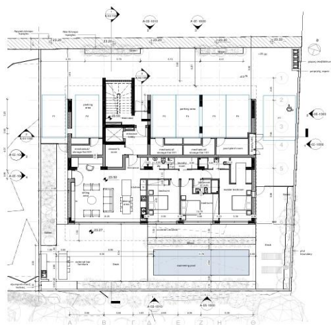
1 Ground Floor Scale: 1 : 100
