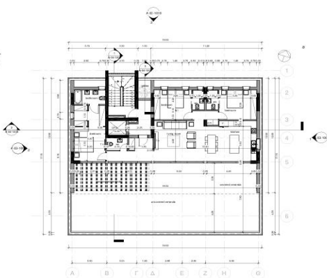
2 1st Floor Scale: 1 : 100
