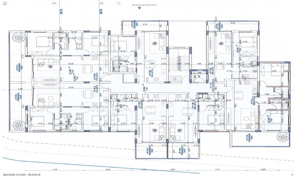
SECOND FLOOR - BLOCK B
