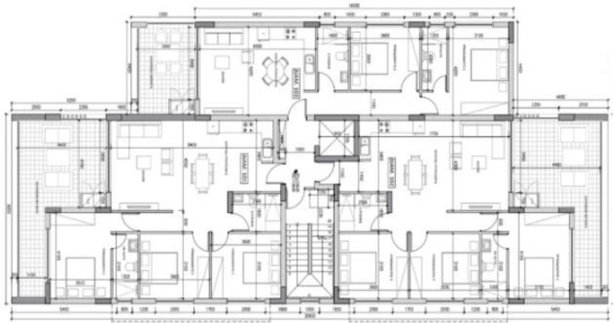
First Floor
