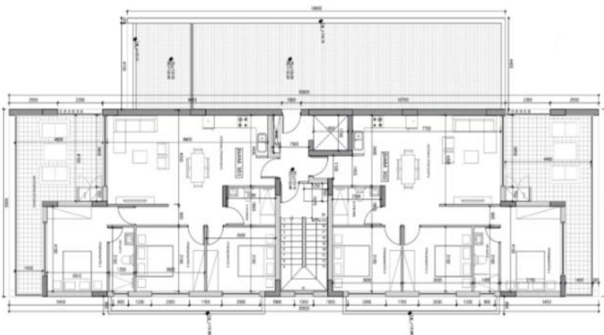
Third Floor
