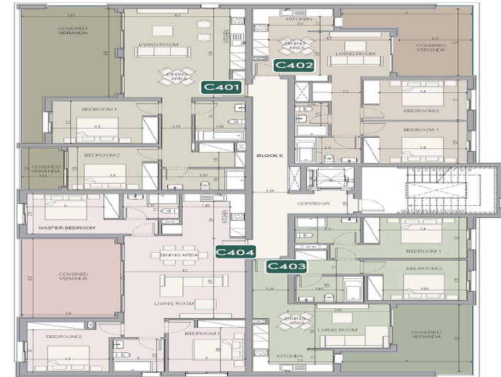
BLOCK C 4th FLOOR PLAN
