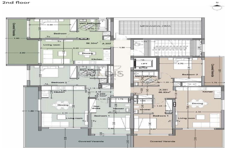
2nd floor
