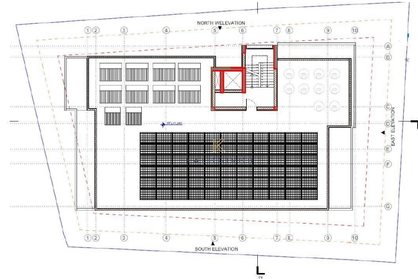
ROOF GARDEN
