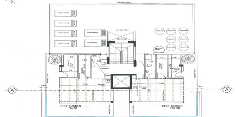
ROOF GARDEN PLAN
