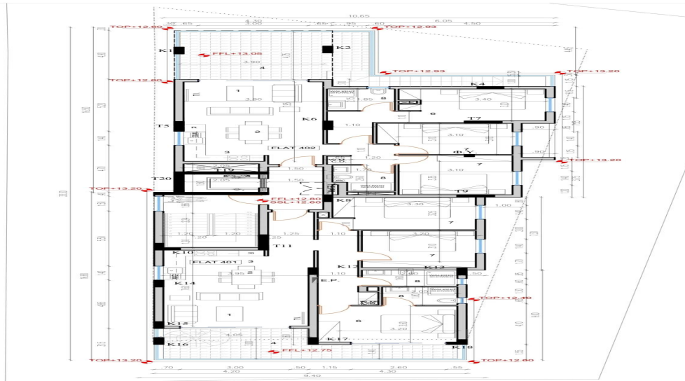
4TH FLOOR PLAN
