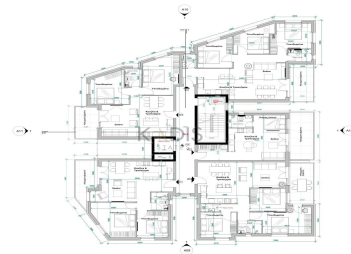
Level 4 1:100
