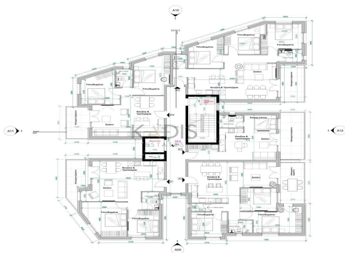
Level 3 1:100
