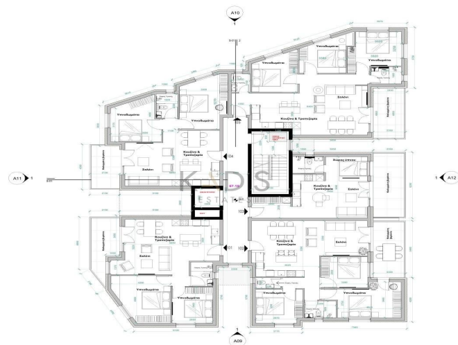
Level 1 1:100
