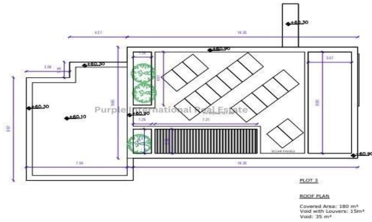
PLOT 3- ROOF PLAN SC 1:100
