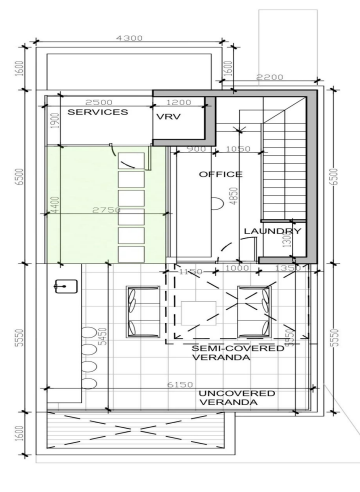
ROOF TERRACE SCALE 1:100
