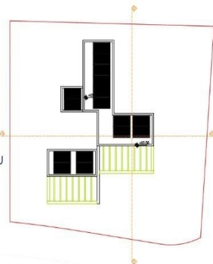
ROOF PLAN
