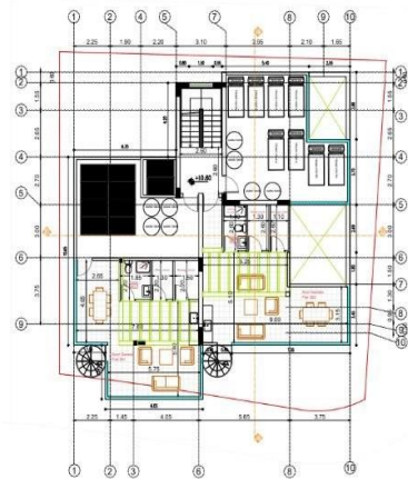
ROOF GARDEN
