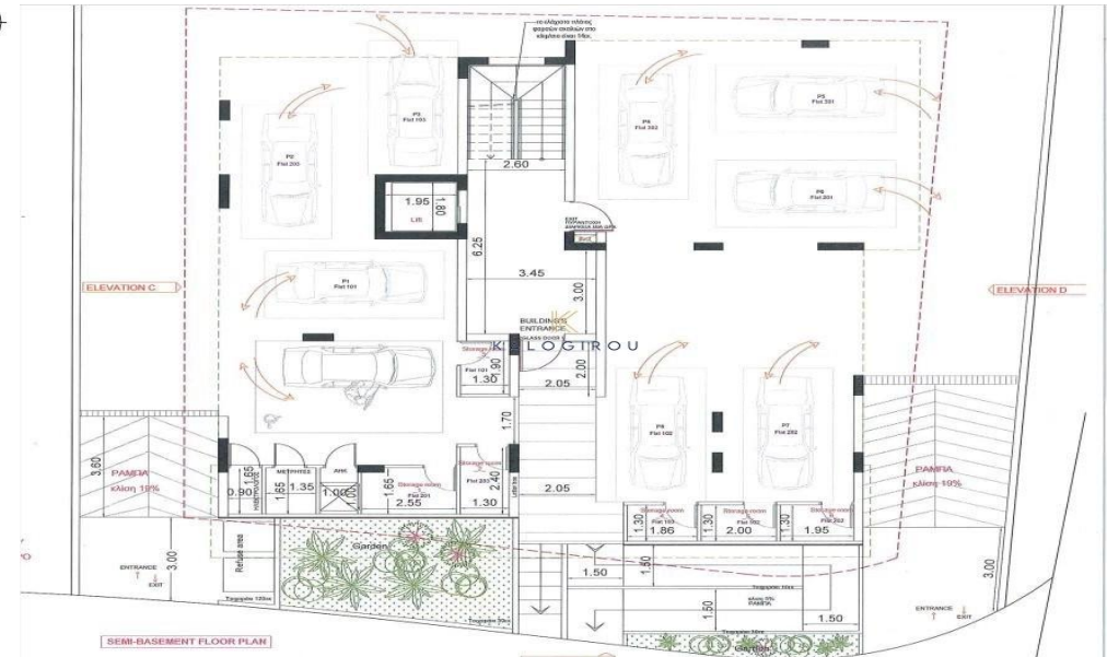
SEMI-BASEMENT FLOOR PLAN
