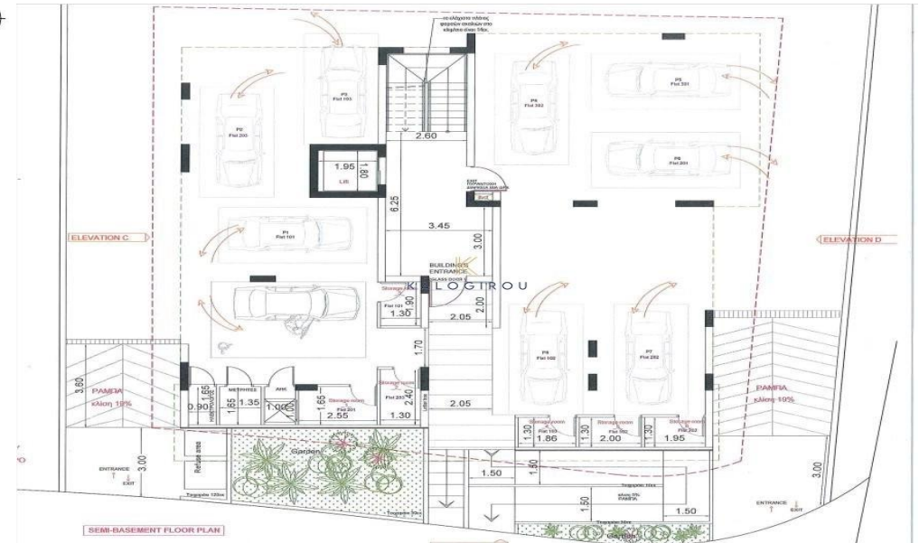
SEMI-BASEMENT FLOOR PLAN
