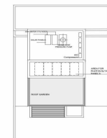
ROOF PLAN 2
