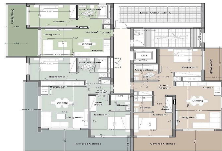
1st floor
