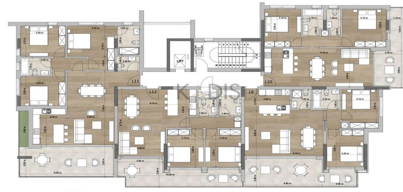
THIRD FLOOR
