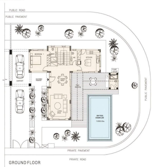
3 BEDROOM VILLA
