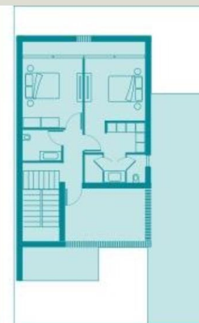
Fist floor
