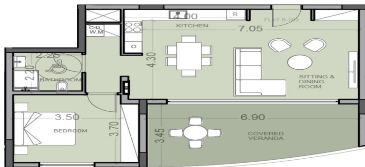
BLOCK B - 2 nd FLOOR APARTMENT 202
