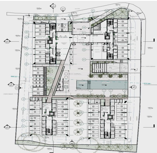
MASTERPLAN GROUND FLOOR
