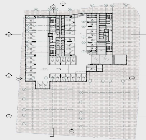
MASTERPLAN BASEMENT
