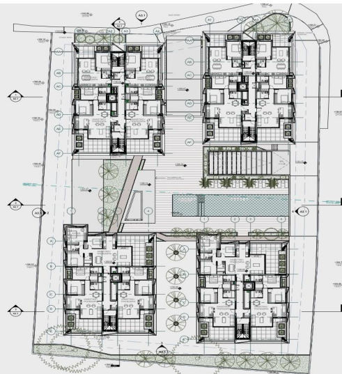
MASTERPLAN LEVEL 1
